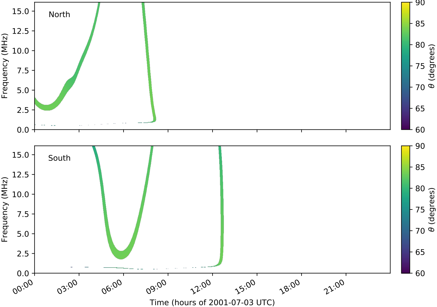
expres_cassini_jupiter_ganymede_isaac_lossc-wid1deg_3kev_20010703_v01.cdf
