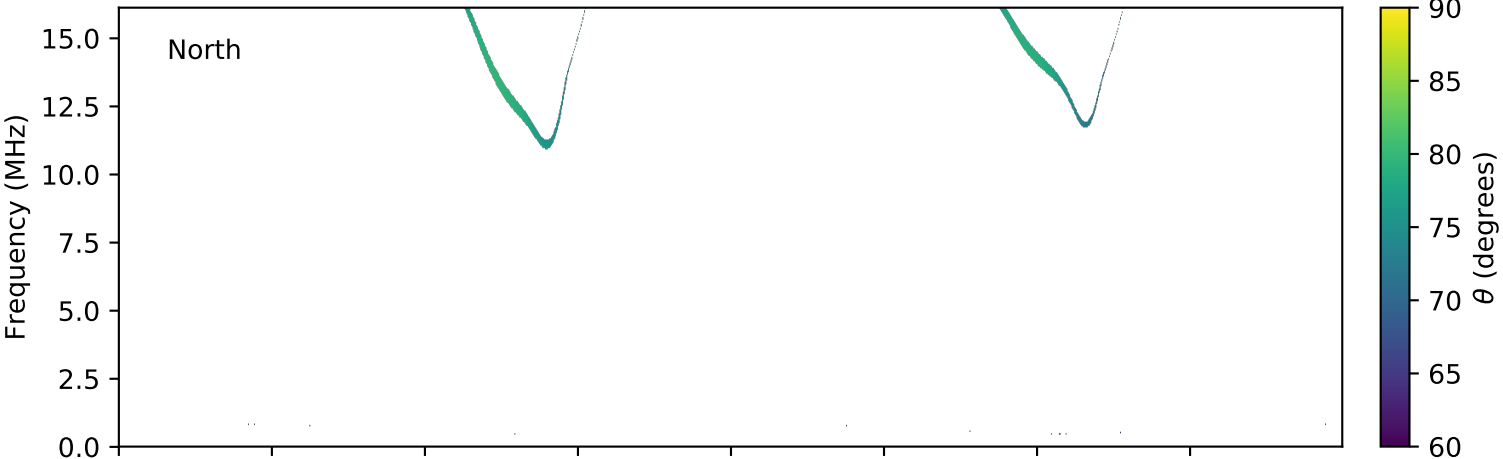
expres_cassini_jupiter_ganymede_isaac_lossc-wid1deg_3kev_20010701_v01.cdf
