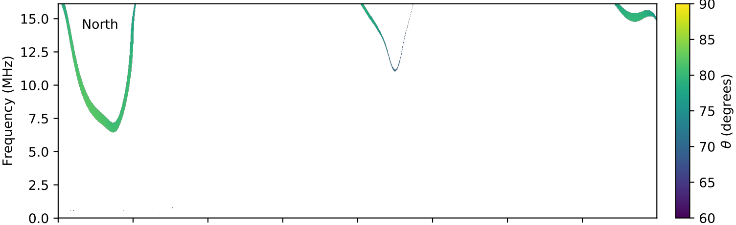
expres_cassini_jupiter_europa_isaac_lossc-wid1deg_3kev_20010731_v01.cdf
