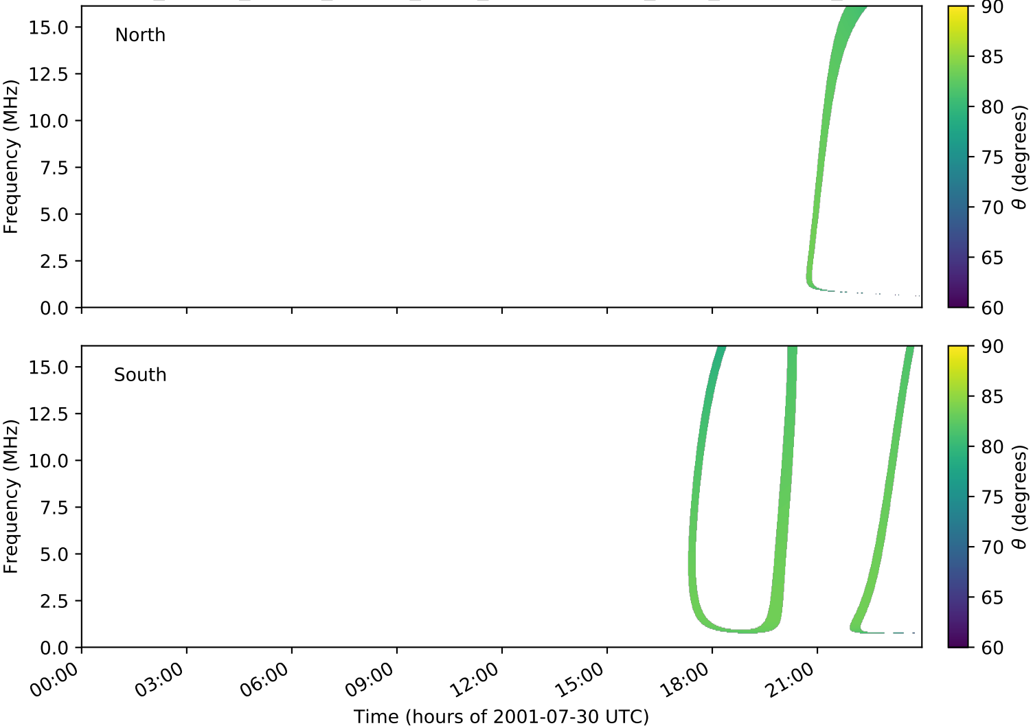
expres_cassini_jupiter_europa_isaac_lossc-wid1deg_3kev_20010730_v01.cdf
