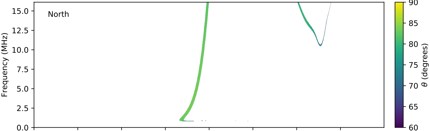
expres_cassini_jupiter_europa_isaac_lossc-wid1deg_3kev_20010727_v01.cdf
