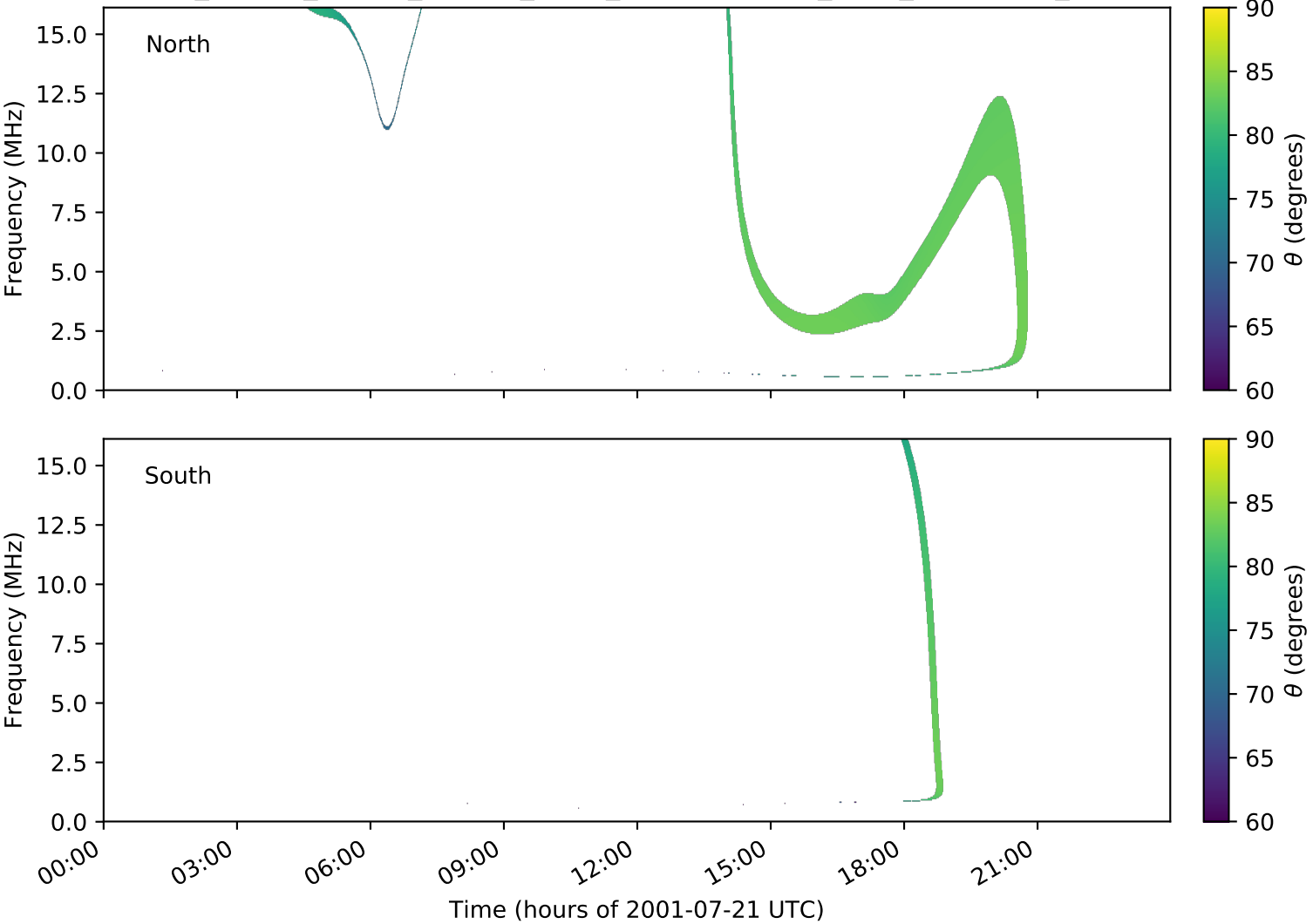
expres_cassini_jupiter_europa_isaac_lossc-wid1deg_3kev_20010721_v01.cdf
