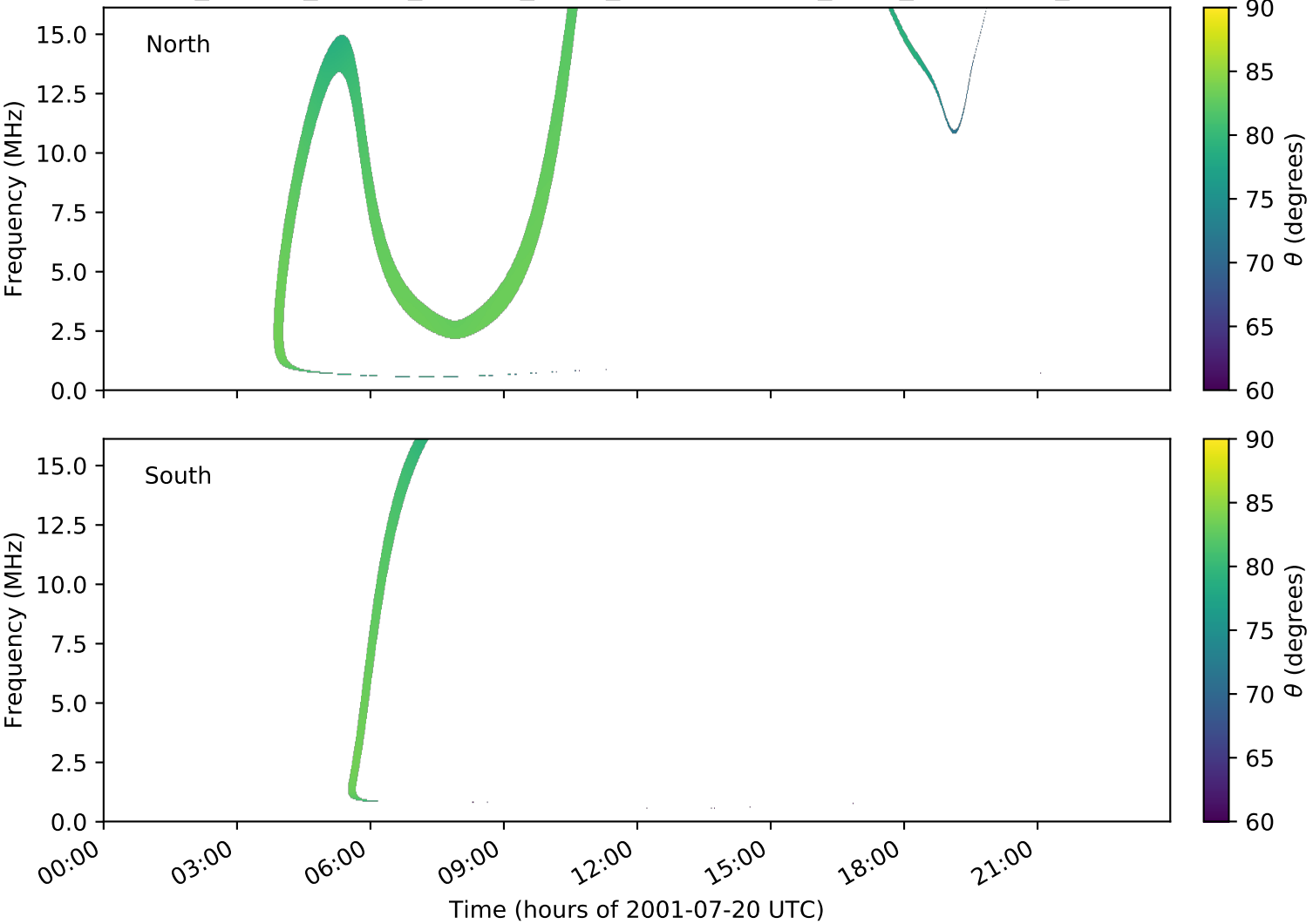
expres_cassini_jupiter_europa_isaac_lossc-wid1deg_3kev_20010720_v01.cdf
