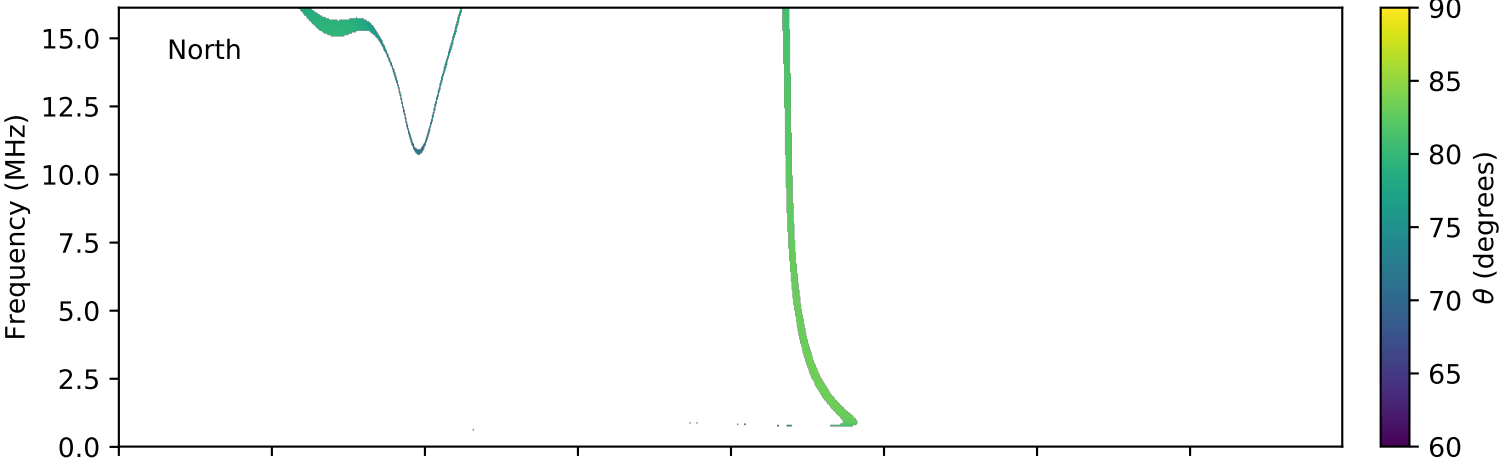
expres_cassini_jupiter_europa_isaac_lossc-wid1deg_3kev_20010714_v01.cdf
