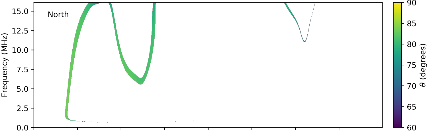
expres_cassini_jupiter_europa_isaac_lossc-wid1deg_3kev_20010713_v01.cdf
