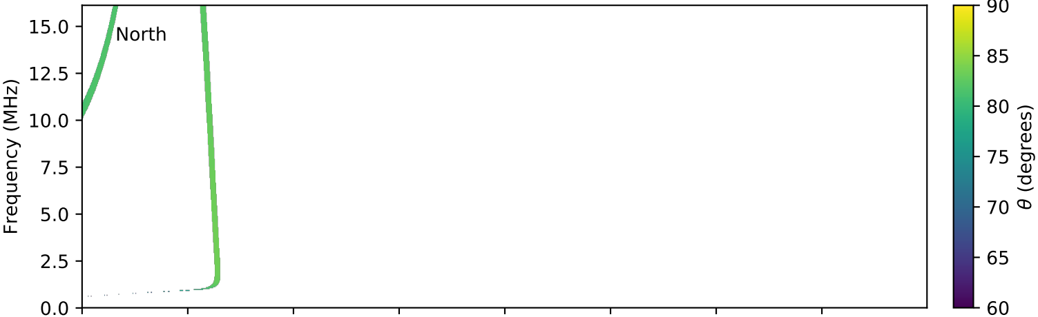
expres_cassini_jupiter_europa_isaac_lossc-wid1deg_3kev_20010711_v01.cdf
