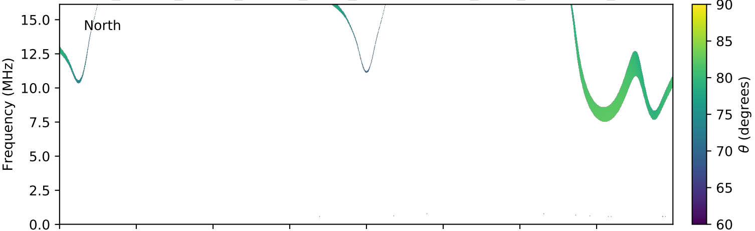
expres_cassini_jupiter_europa_isaac_lossc-wid1deg_3kev_20010710_v01.cdf
