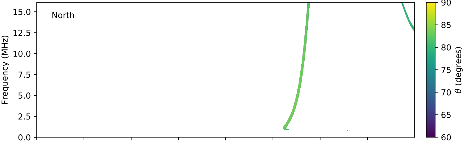
expres_cassini_jupiter_europa_isaac_lossc-wid1deg_3kev_20010709_v01.cdf
