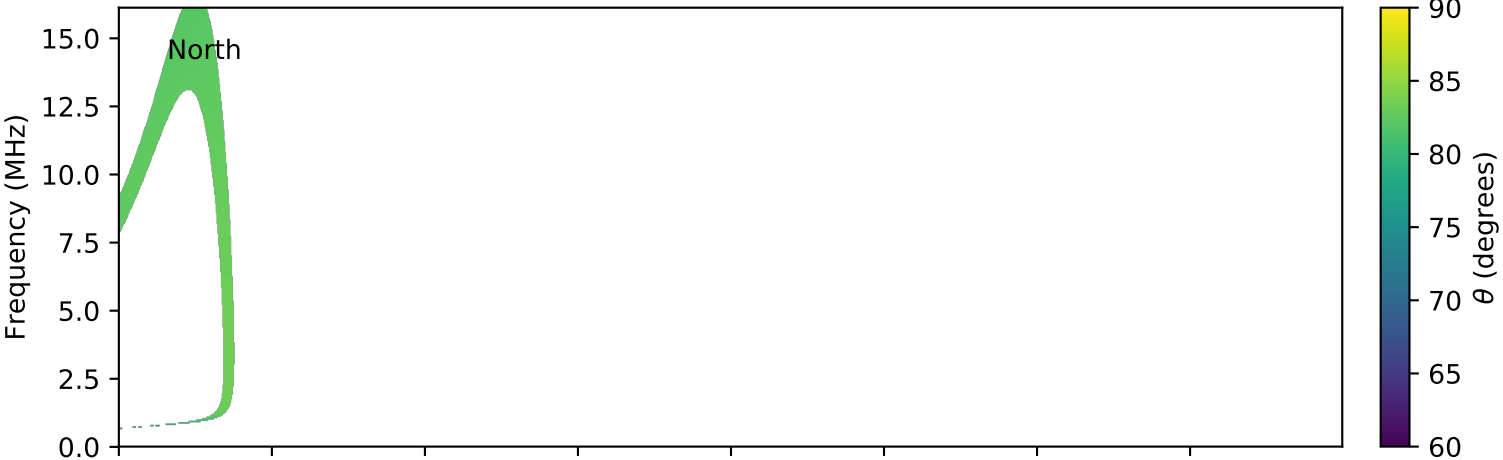
expres_cassini_jupiter_europa_isaac_lossc-wid1deg_3kev_20010704_v01.cdf
