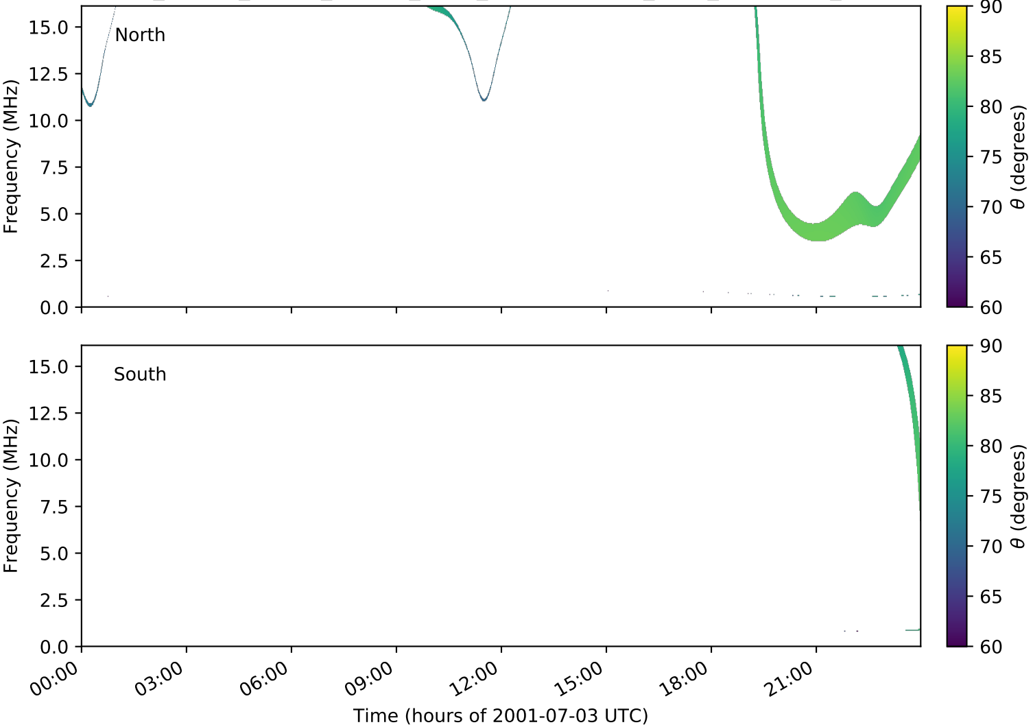
expres_cassini_jupiter_europa_isaac_lossc-wid1deg_3kev_20010703_v01.cdf
