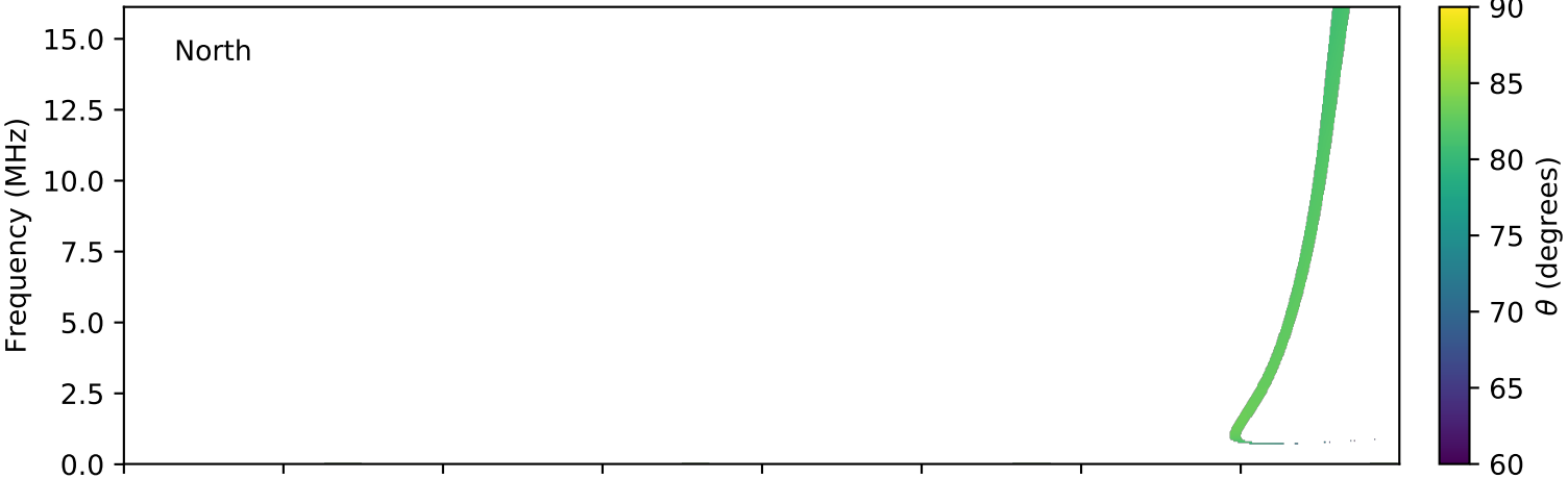
expres_cassini_jupiter_io_isaac_lossc-wid1deg_3kev_20010630_v01.cdf
