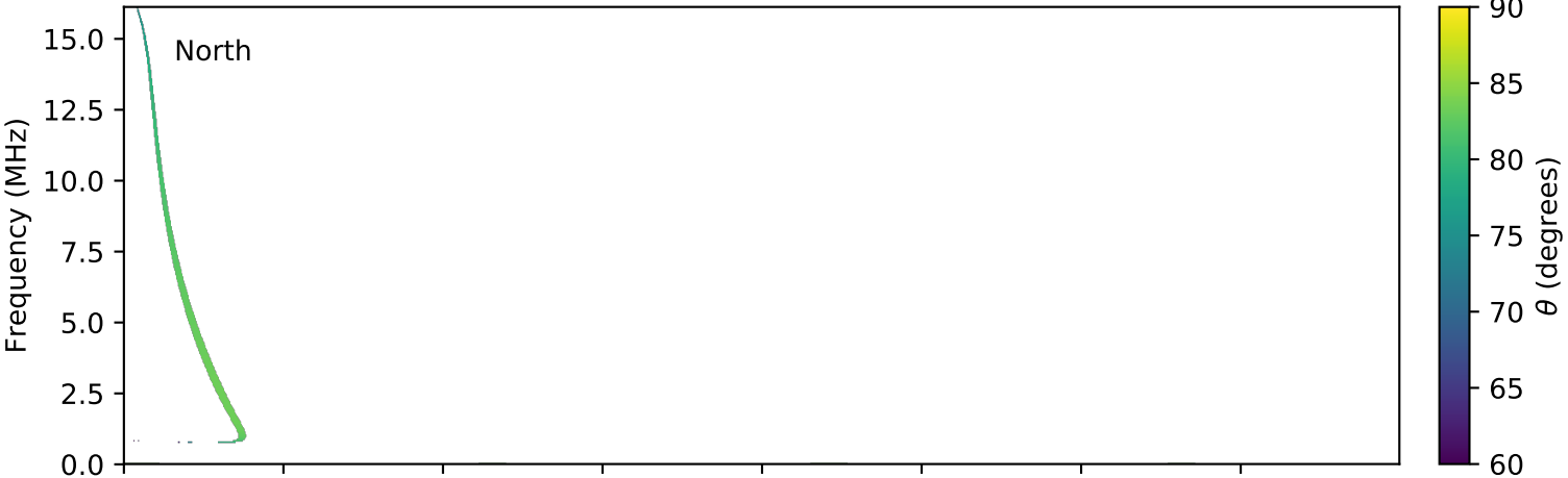
expres_cassini_jupiter_io_isaac_lossc-wid1deg_3kev_20010628_v01.cdf
