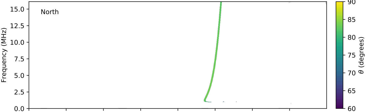
expres_cassini_jupiter_io_isaac_lossc-wid1deg_3kev_20010625_v01.cdf
