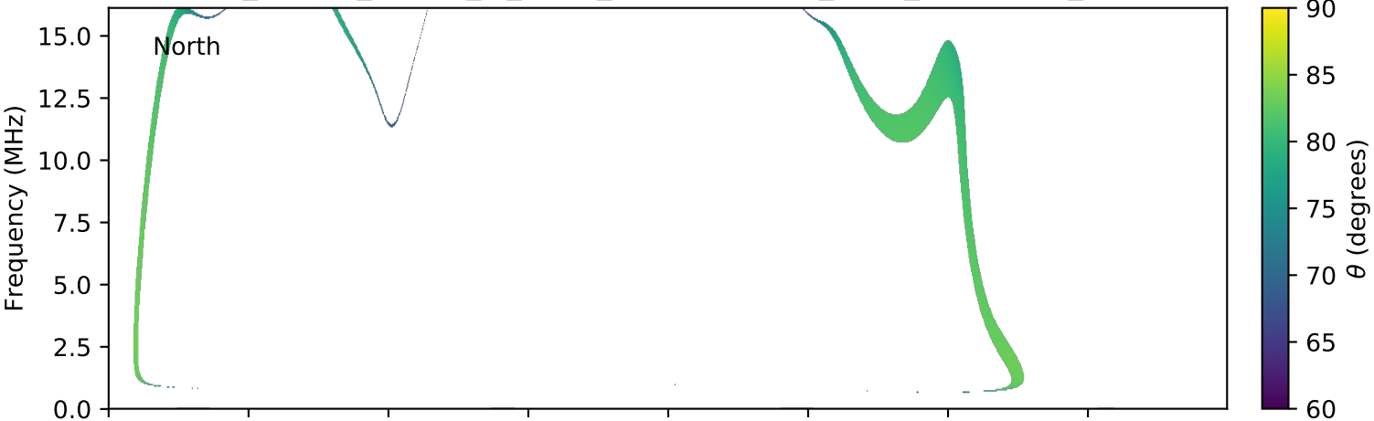
expres_cassini_jupiter_io_isaac_lossc-wid1deg_3kev_20010622_v01.cdf
