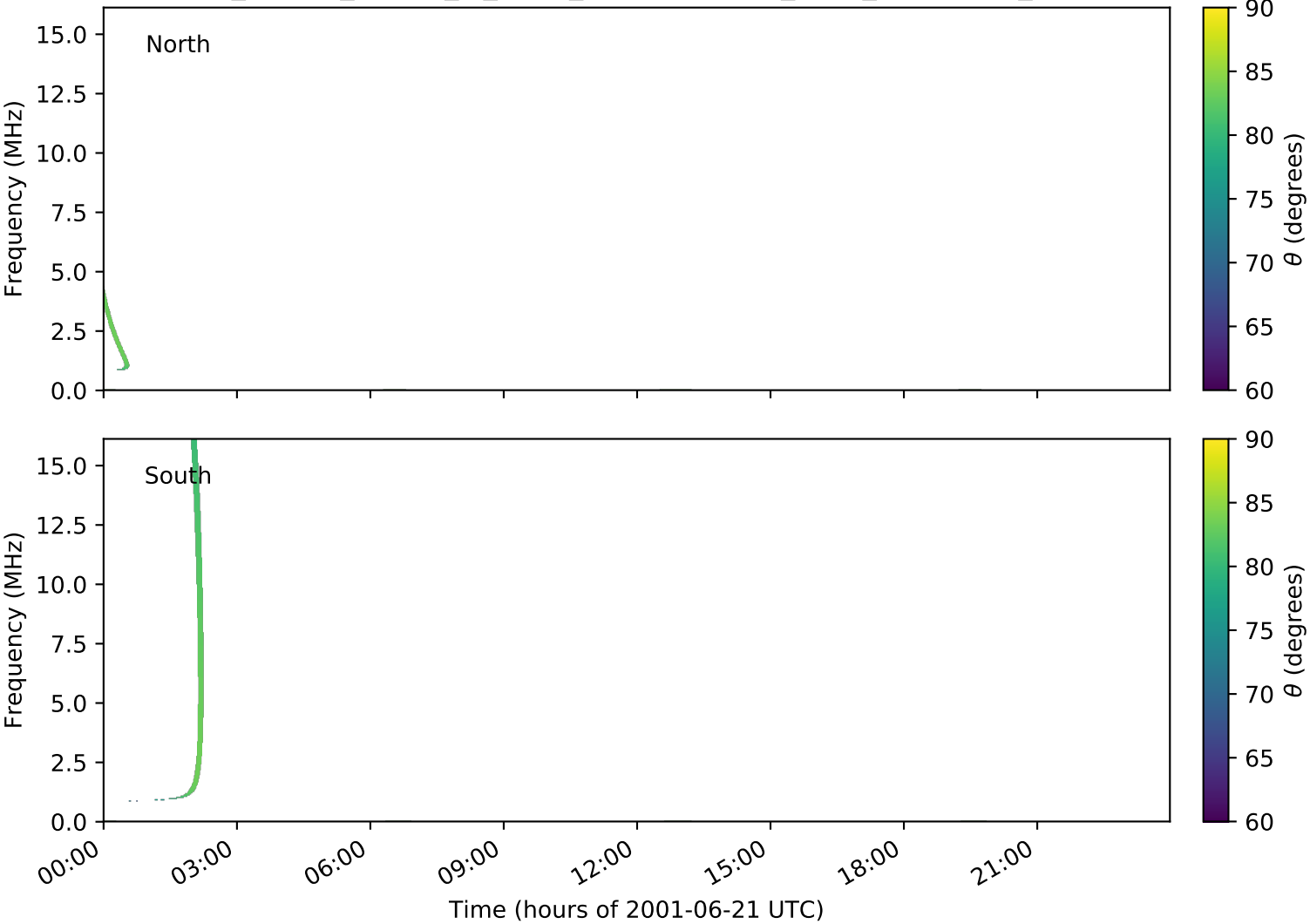
expres_cassini_jupiter_io_isaac_lossc-wid1deg_3kev_20010621_v01.cdf
