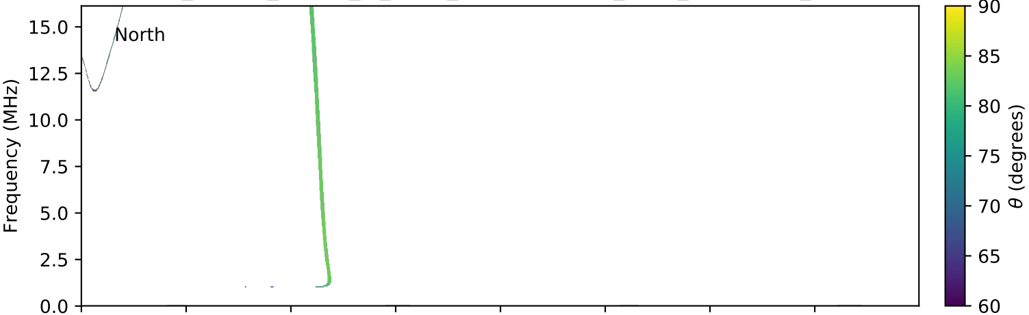
expres_cassini_jupiter_io_isaac_lossc-wid1deg_3kev_20010619_v01.cdf
