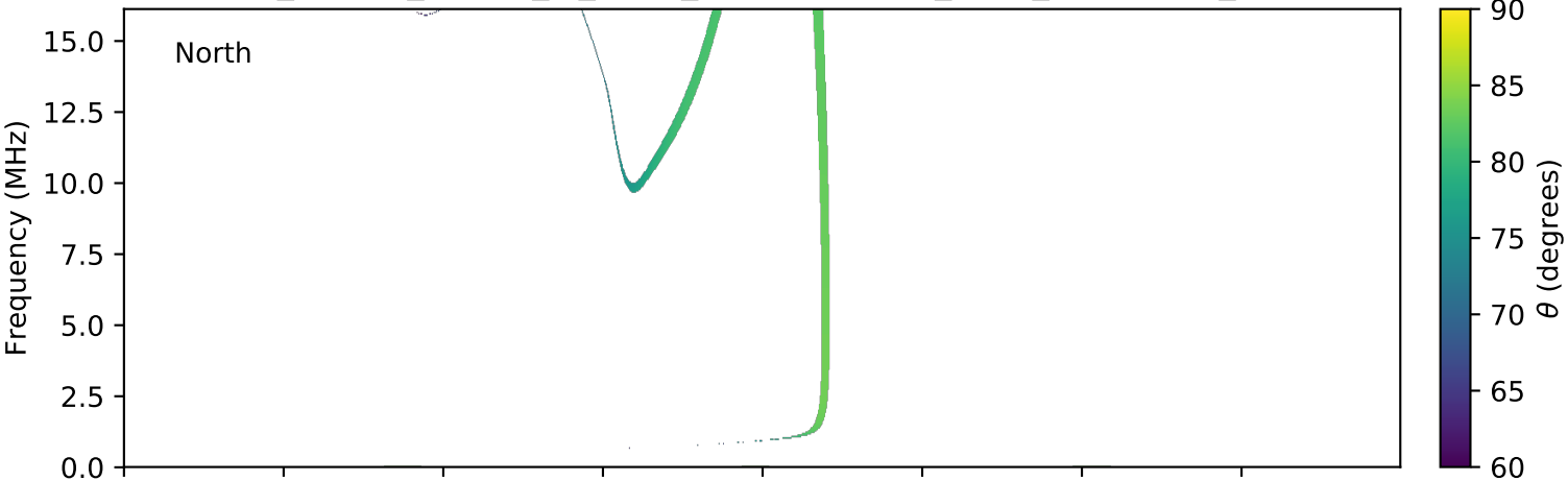
expres_cassini_jupiter_io_isaac_lossc-wid1deg_3kev_20010617_v01.cdf
