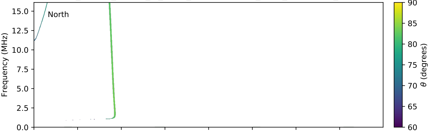
expres_cassini_jupiter_io_isaac_lossc-wid1deg_3kev_20010612_v01.cdf
