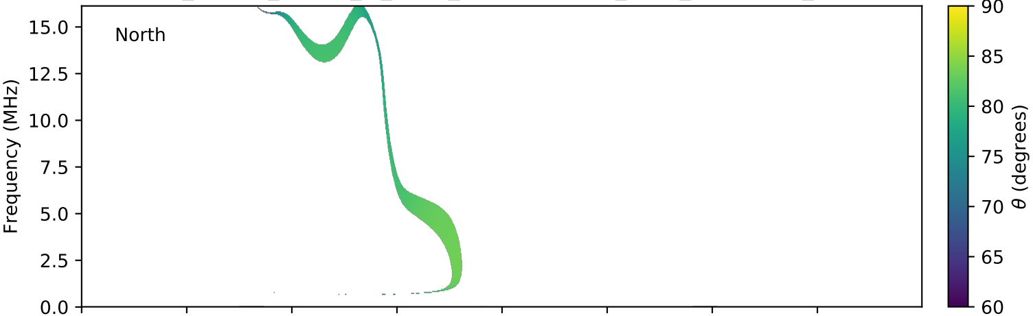
expres_cassini_jupiter_io_isaac_lossc-wid1deg_3kev_20010610_v01.cdf
