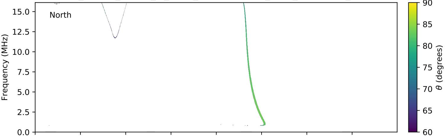
expres_cassini_jupiter_io_isaac_lossc-wid1deg_3kev_20010608_v01.cdf
