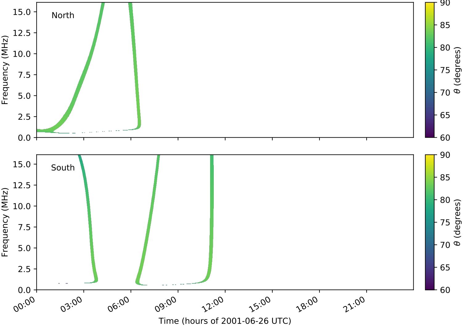
expres_cassini_jupiter_ganymede_isaac_lossc-wid1deg_3kev_20010626_v01.cdf
