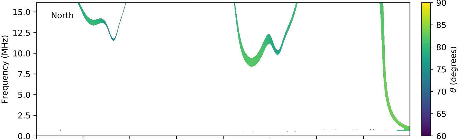
expres_cassini_jupiter_ganymede_isaac_lossc-wid1deg_3kev_20010625_v01.cdf
