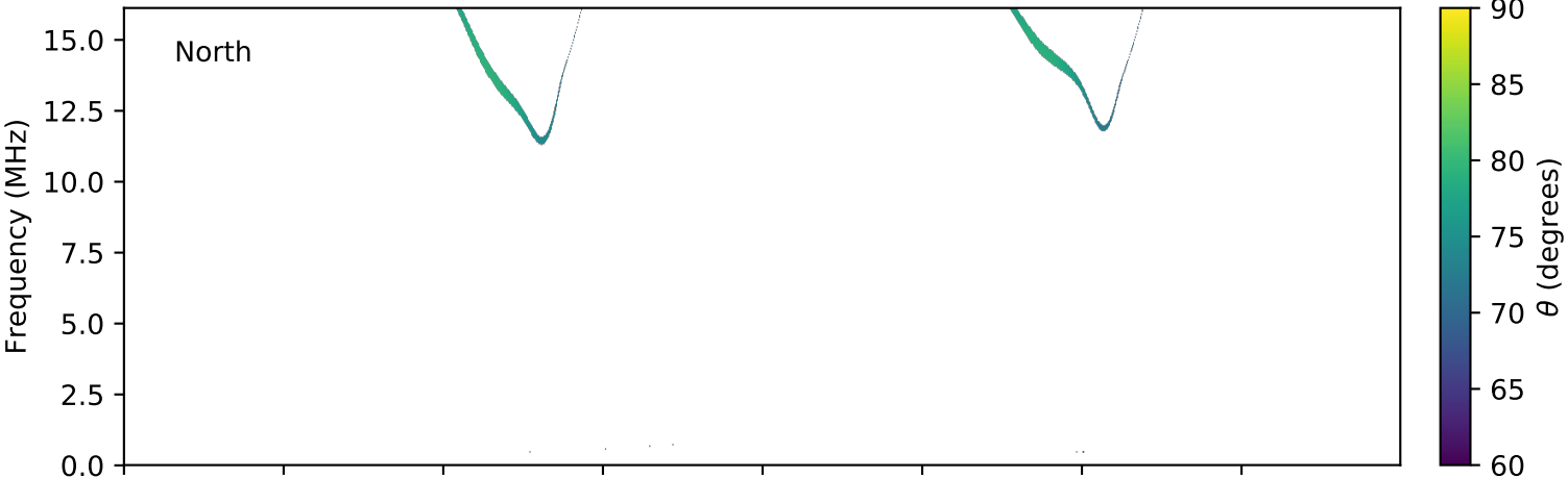
expres_cassini_jupiter_ganymede_isaac_lossc-wid1deg_3kev_20010624_v01.cdf
