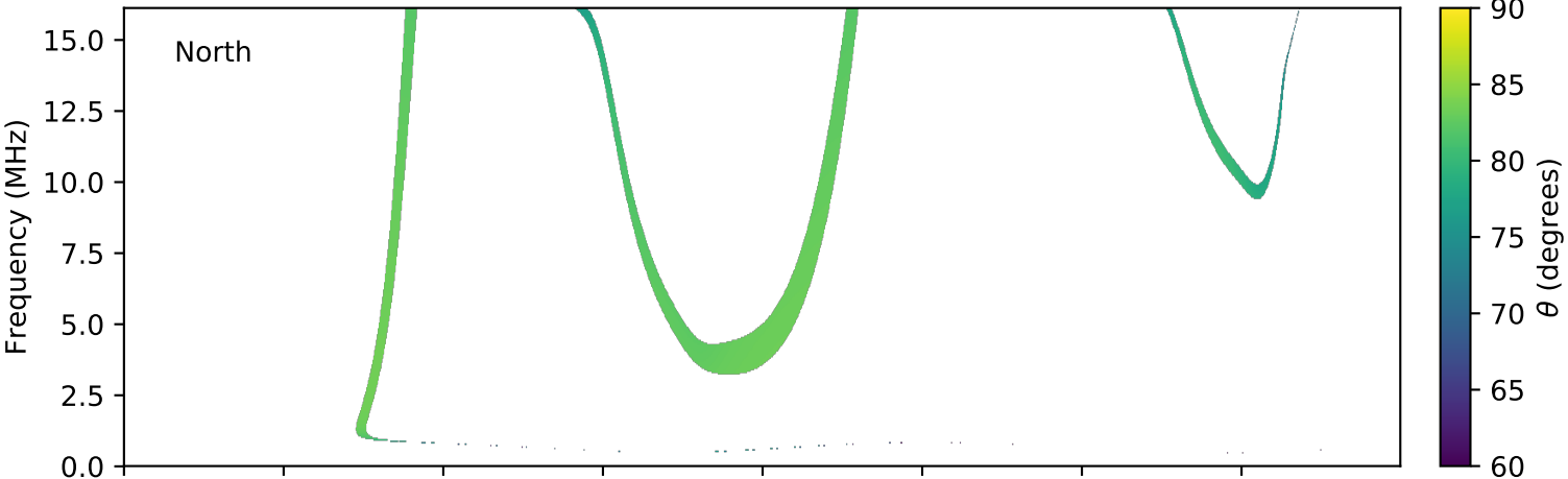
expres_cassini_jupiter_ganymede_isaac_lossc-wid1deg_3kev_20010623_v01.cdf
