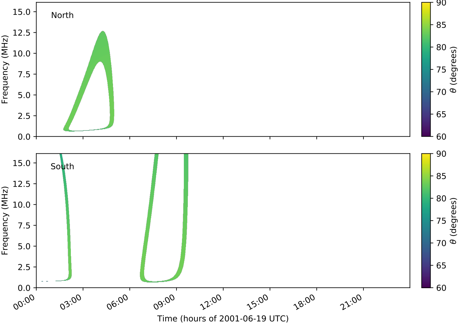
expres_cassini_jupiter_ganymede_isaac_lossc-wid1deg_3kev_20010619_v01.cdf
