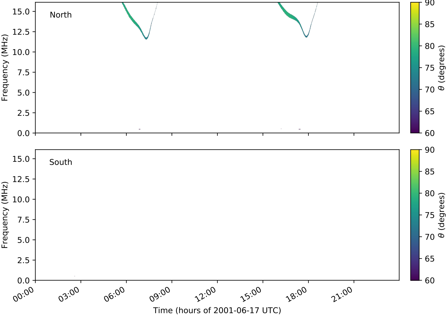
expres_cassini_jupiter_ganymede_isaac_lossc-wid1deg_3kev_20010617_v01.cdf
