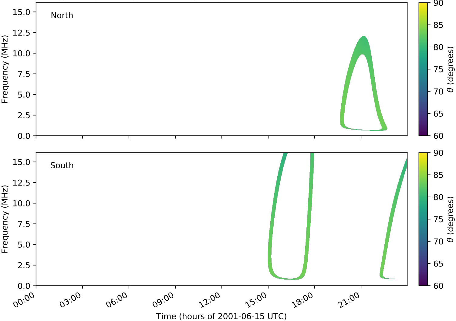
expres_cassini_jupiter_ganymede_isaac_lossc-wid1deg_3kev_20010615_v01.cdf
