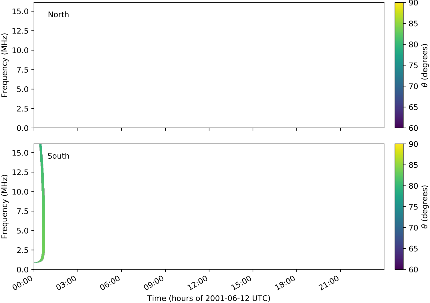
expres_cassini_jupiter_ganymede_isaac_lossc-wid1deg_3kev_20010612_v01.cdf
