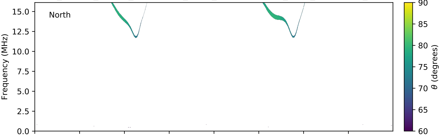
expres_cassini_jupiter_ganymede_isaac_lossc-wid1deg_3kev_20010610_v01.cdf
