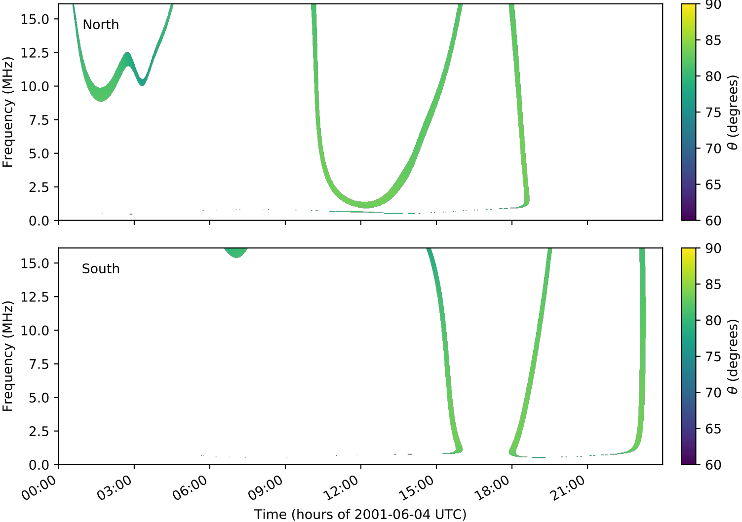
expres_cassini_jupiter_ganymede_isaac_lossc-wid1deg_3kev_20010604_v01.cdf
