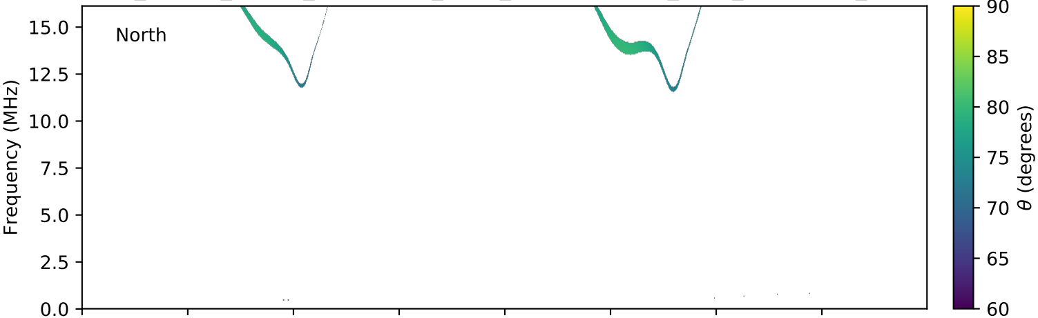
expres_cassini_jupiter_ganymede_isaac_lossc-wid1deg_3kev_20010603_v01.cdf
