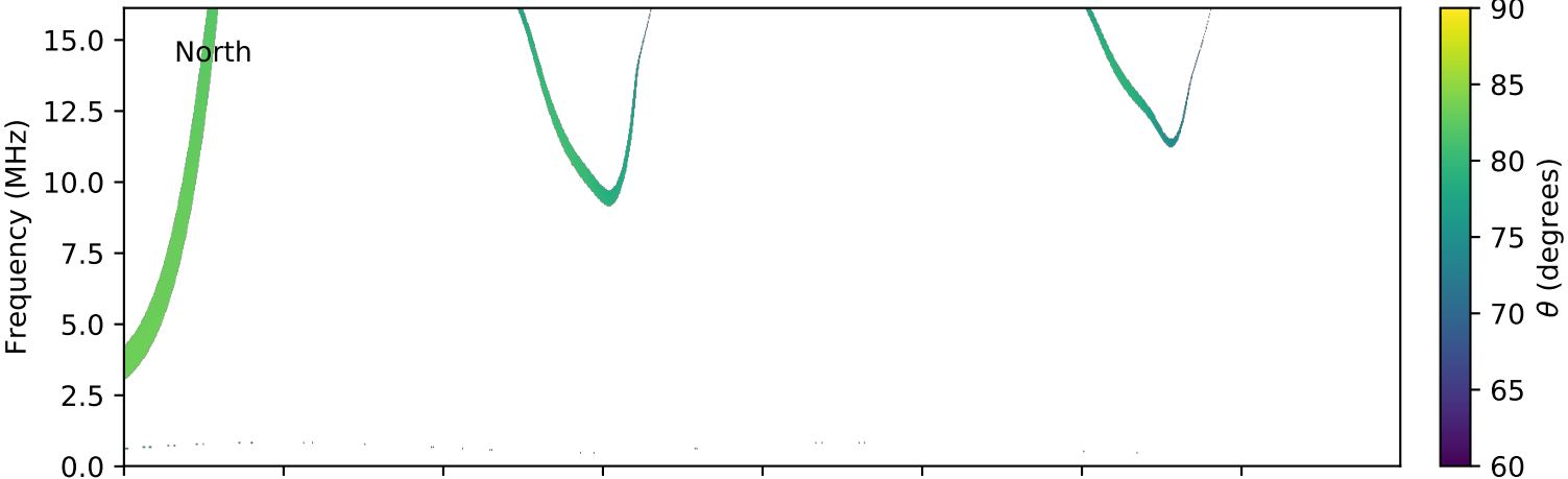
expres_cassini_jupiter_ganymede_isaac_lossc-wid1deg_3kev_20010602_v01.cdf
