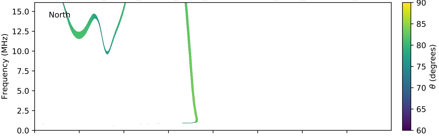
expres_cassini_jupiter_europa_isaac_lossc-wid1deg_3kev_20010630_v01.cdf
