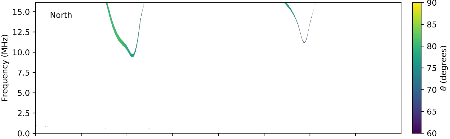
expres_cassini_jupiter_europa_isaac_lossc-wid1deg_3kev_20010629_v01.cdf
