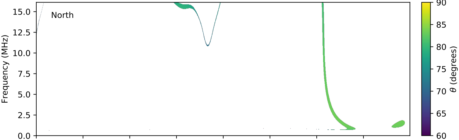
expres_cassini_jupiter_europa_isaac_lossc-wid1deg_3kev_20010626_v01.cdf
