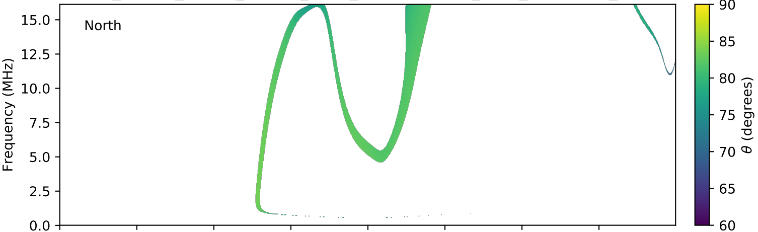
expres_cassini_jupiter_europa_isaac_lossc-wid1deg_3kev_20010625_v01.cdf
