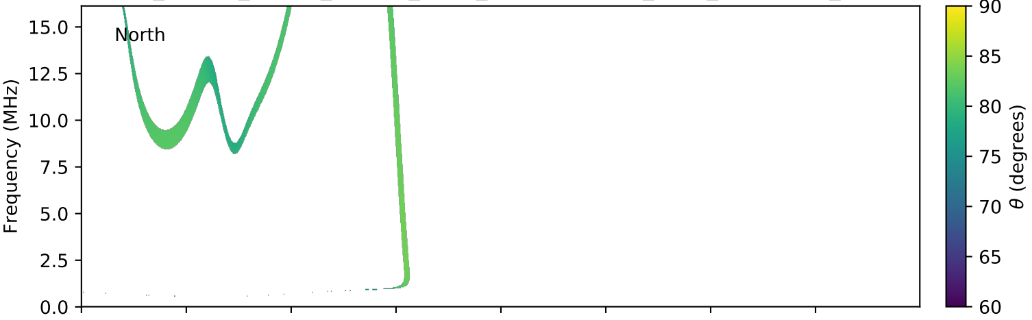
expres_cassini_jupiter_europa_isaac_lossc-wid1deg_3kev_20010623_v01.cdf
