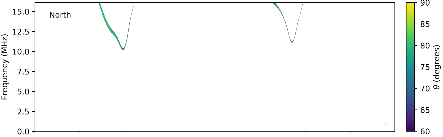
expres_cassini_jupiter_europa_isaac_lossc-wid1deg_3kev_20010622_v01.cdf
