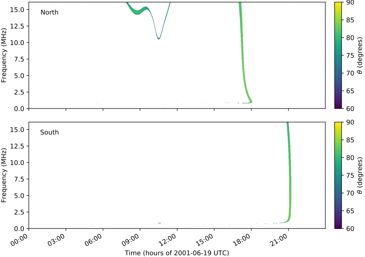
expres_cassini_jupiter_europa_isaac_lossc-wid1deg_3kev_20010619_v01.cdf
