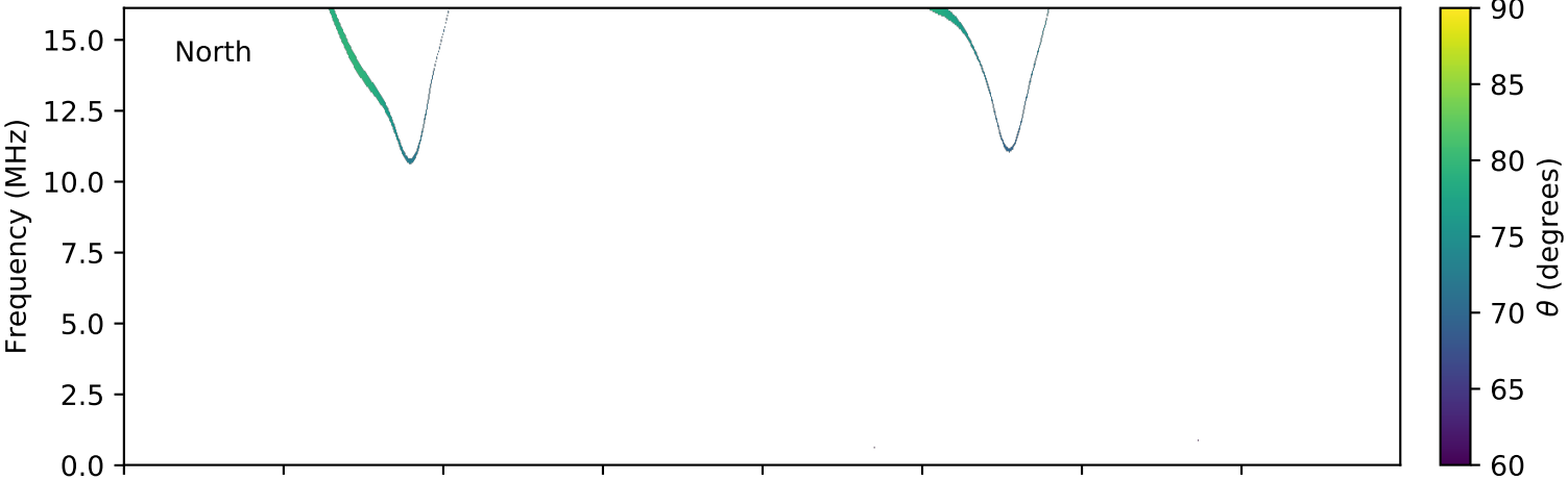
expres_cassini_jupiter_europa_isaac_lossc-wid1deg_3kev_20010615_v01.cdf
