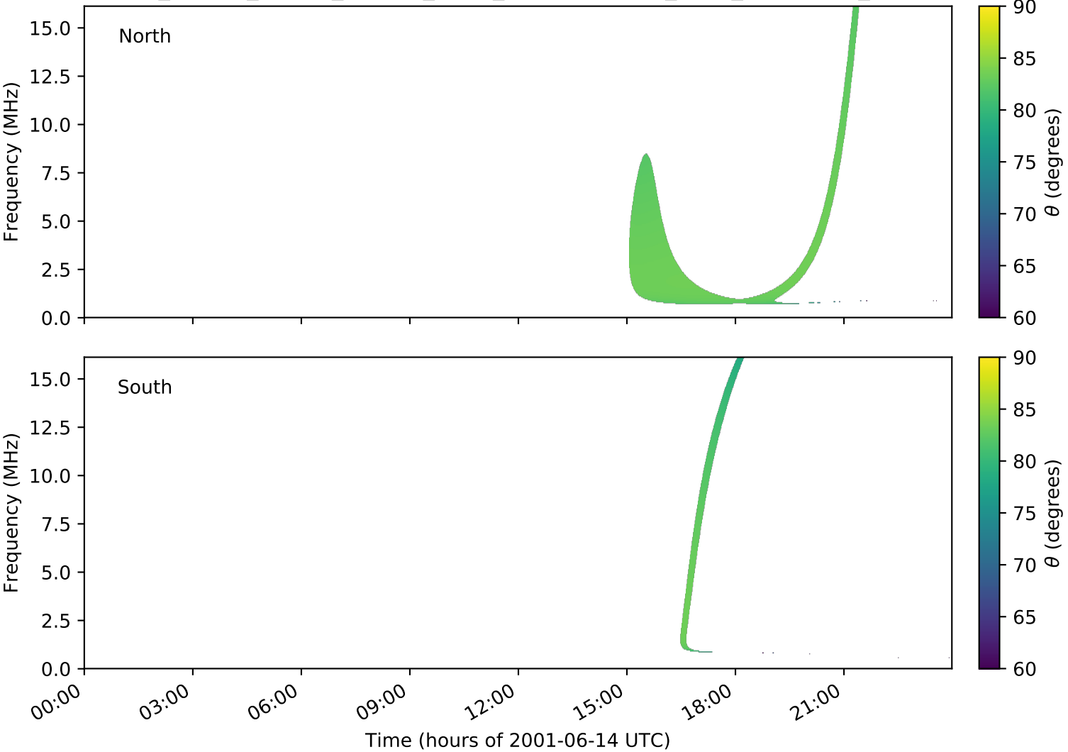
expres_cassini_jupiter_europa_isaac_lossc-wid1deg_3kev_20010614_v01.cdf
