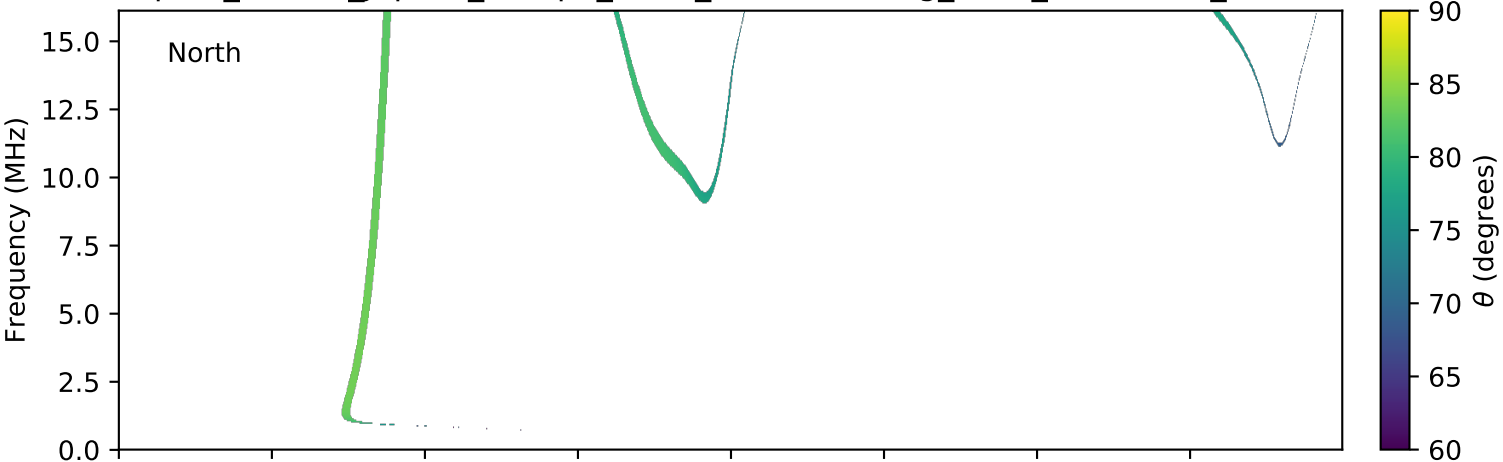
expres_cassini_jupiter_europa_isaac_lossc-wid1deg_3kev_20010611_v01.cdf
