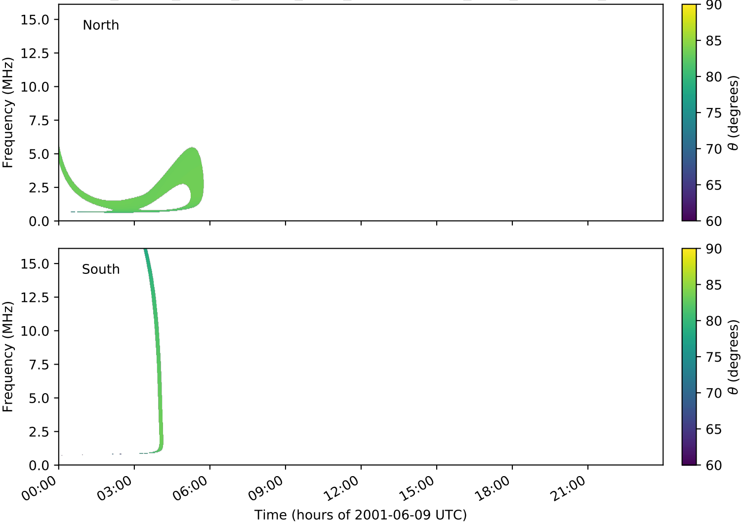
expres_cassini_jupiter_europa_isaac_lossc-wid1deg_3kev_20010609_v01.cdf
