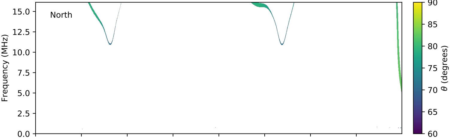
expres_cassini_jupiter_europa_isaac_lossc-wid1deg_3kev_20010608_v01.cdf
