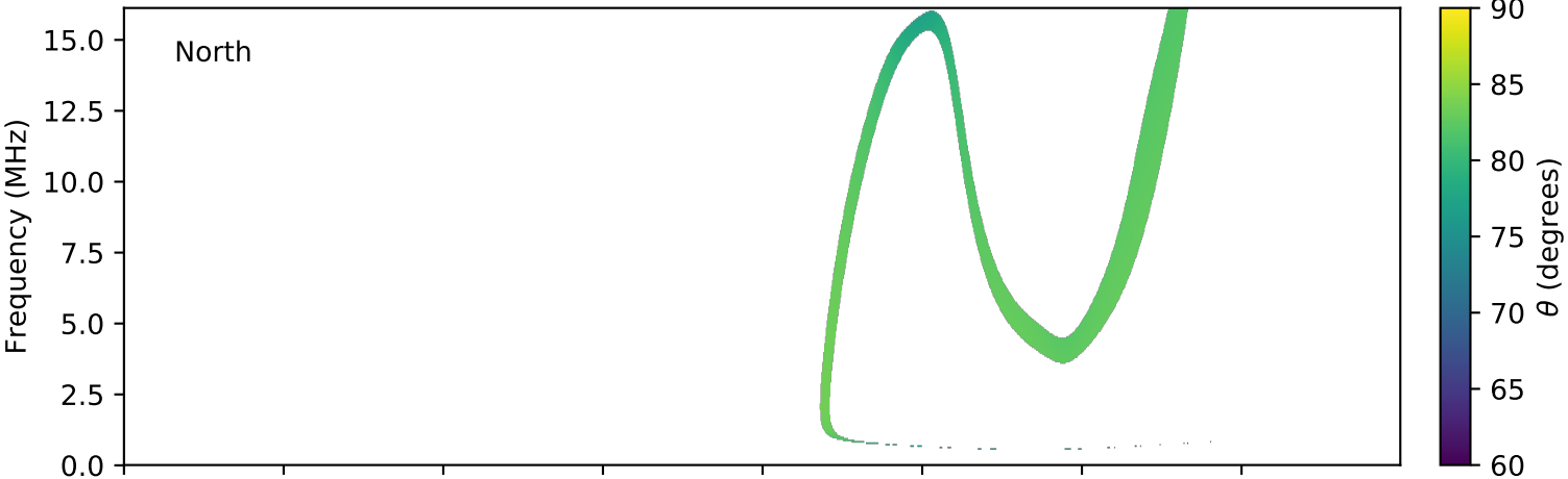
expres_cassini_jupiter_europa_isaac_lossc-wid1deg_3kev_20010607_v01.cdf
