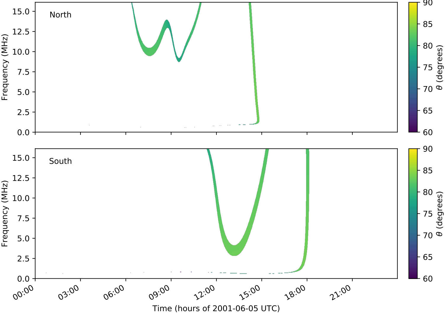
expres_cassini_jupiter_europa_isaac_lossc-wid1deg_3kev_20010605_v01.cdf
